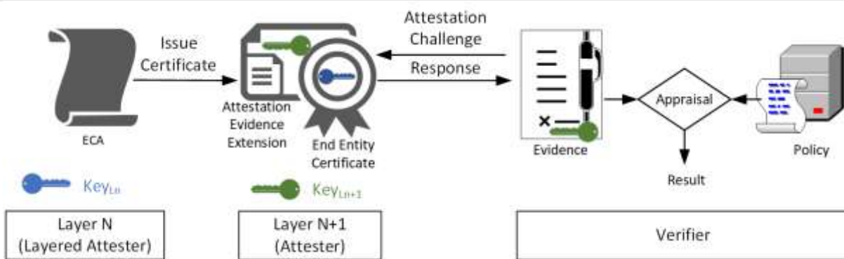
Figure 11: Layered Attestation
