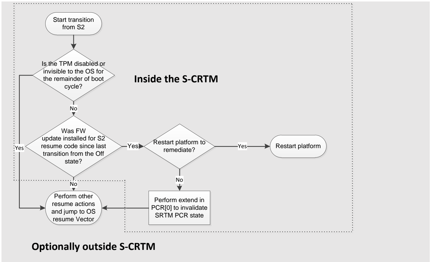
Figure 11 Firmware Actions for S2 Resume
