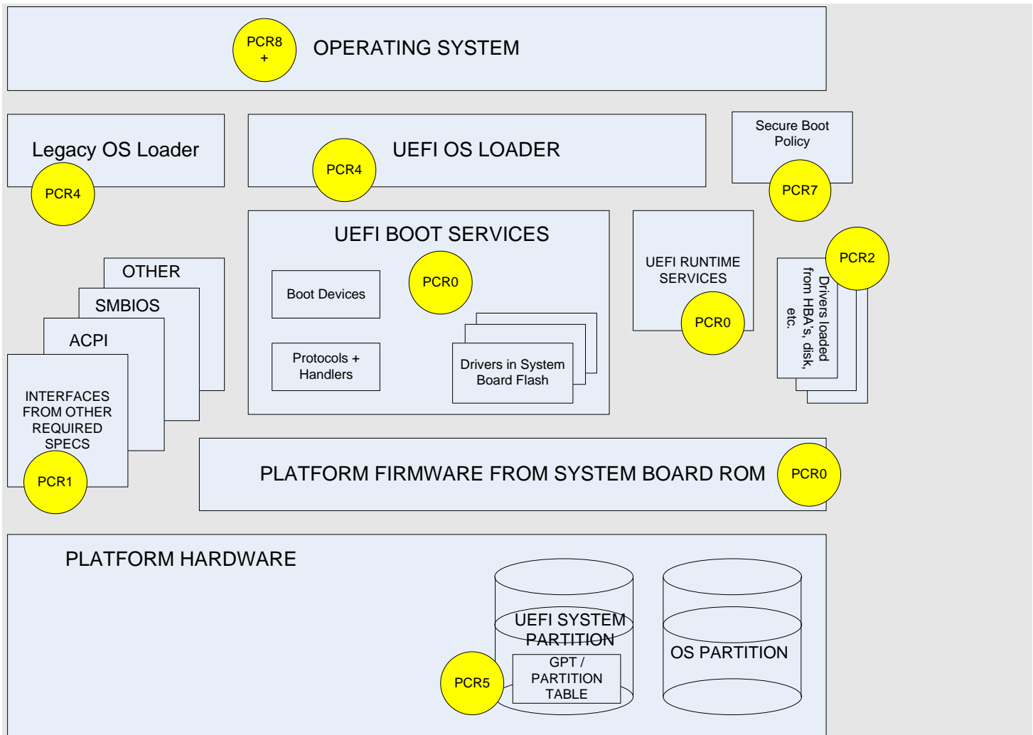
Figure 6 PCR Mapping of UEFI Components
