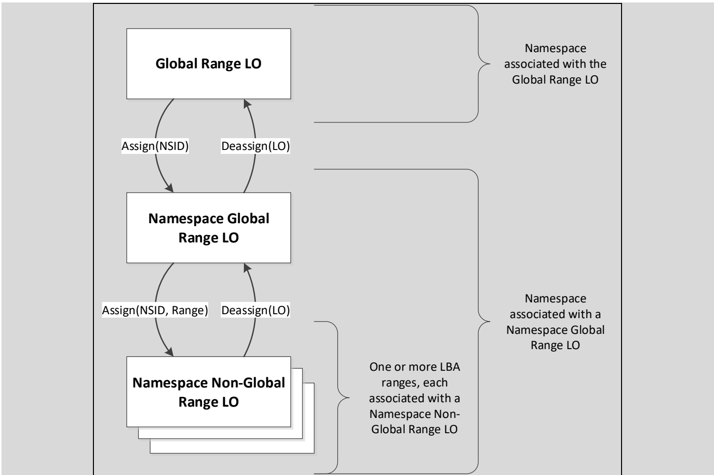
Figure 3 - Flows in Namespace Associations with Locking Objects
