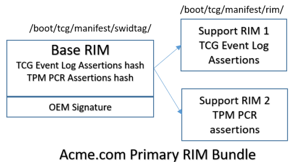
Figure 1: RIM Bundle files illustrated on a Linux based system
