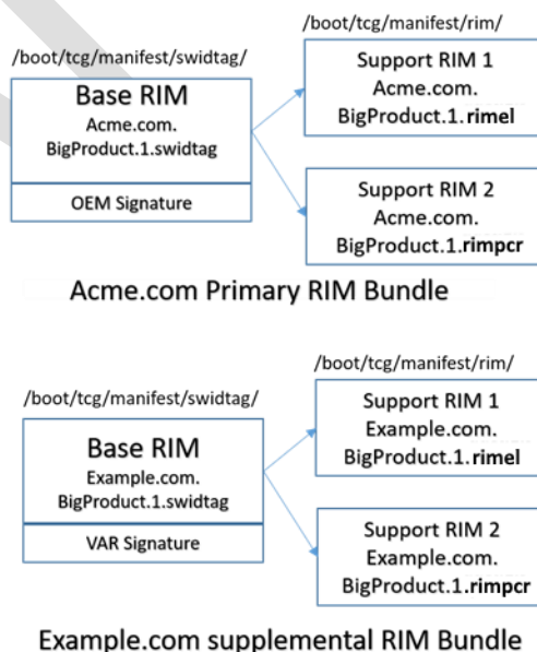
Figure 2 RIM Bundle Collection with Bundle added by a VAR
